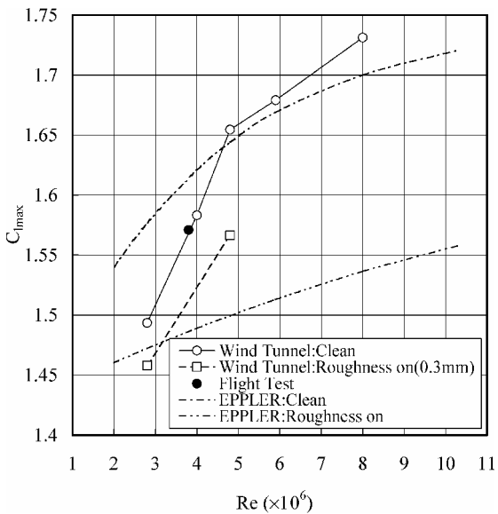
Fig. 11 Effect of Reynolds number on maximum lift coefficient.
