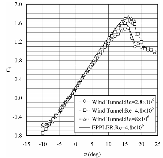
Fig. 10 Comparison of theoretical and experimental (low-speed wind tunnel) lift curves.
