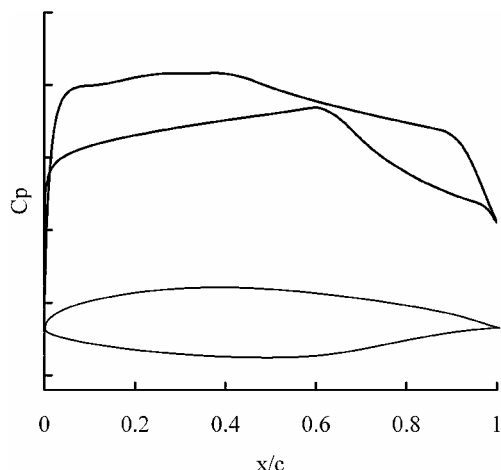
Fig. 1 SHM-1 airfoil shape and pressure distribution.
