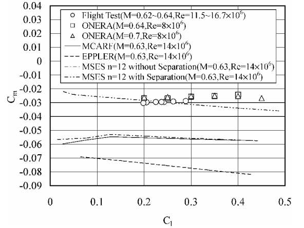
Fig. 14 Comparison of theoretical and experimental (flight and transonic wind tunnel) pitching moment coefficients.
