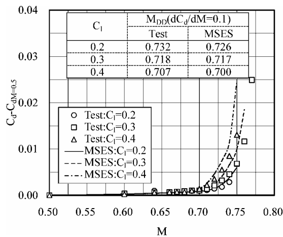
Fig. 17 Comparison of theoretical and experimental (transonic wind tunnel) drag-divergence Mach numbers for Re = 8.0 \times 10^6 with transition fixed.
