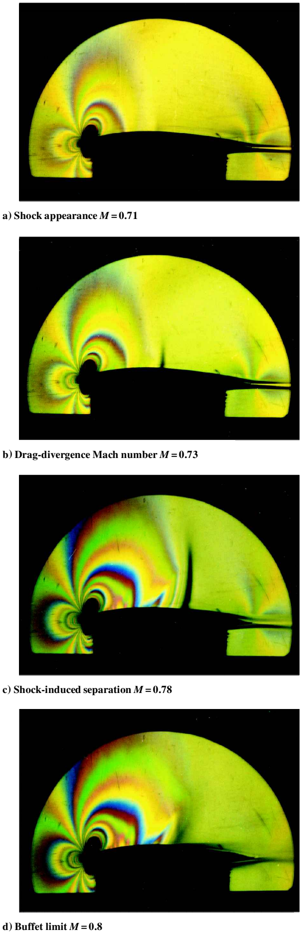
Fig. 18 Schlieren photographs, Re = 8 \times 10^6 and \alpha = 0.5 deg.
